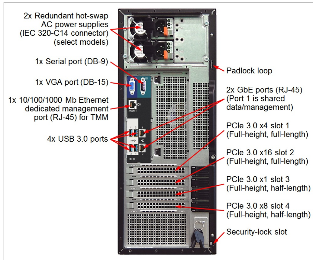
Figure 3. ThinkServer TS460 rear view
