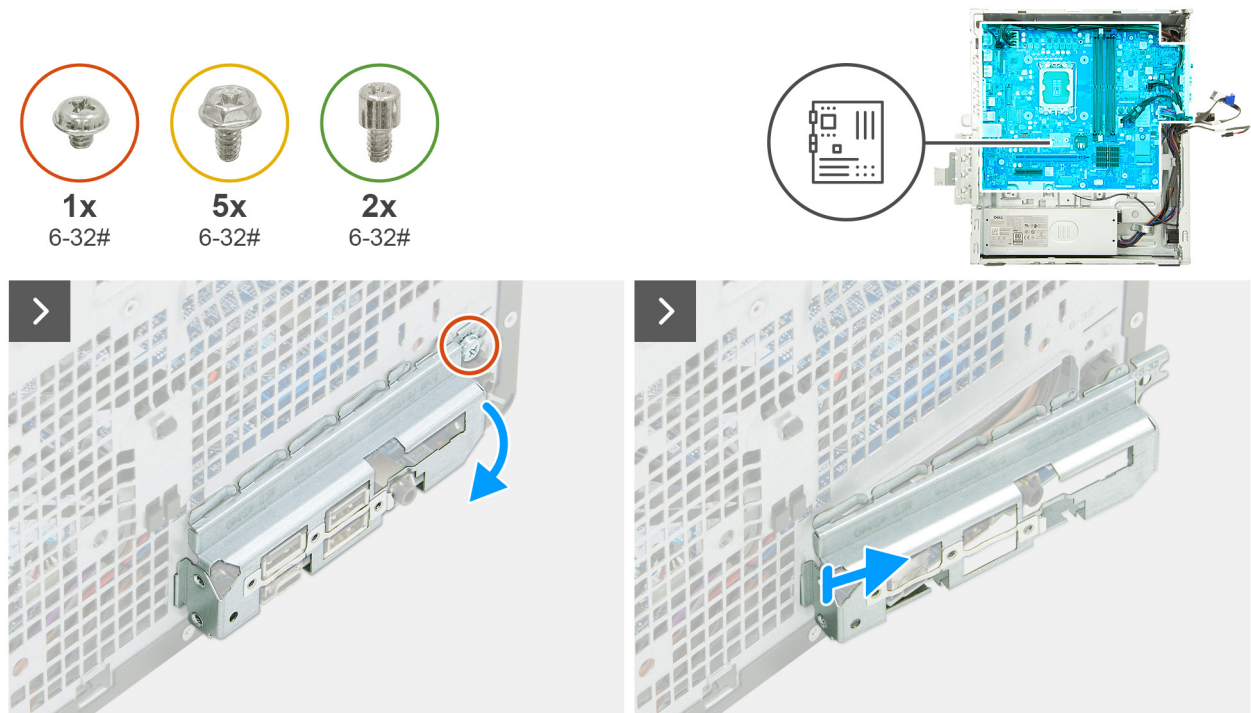
Figure 97. Removing the system board
