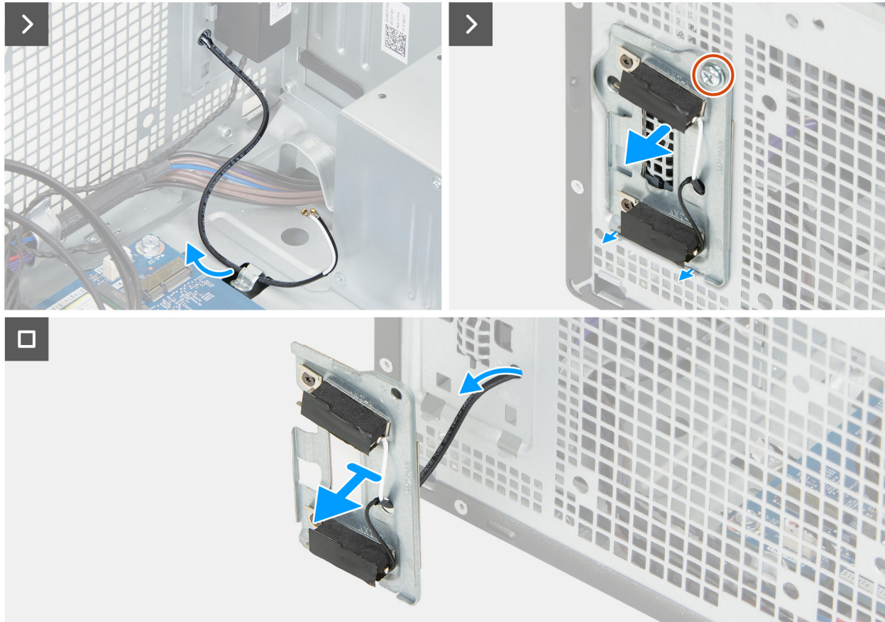
Figure 86. Removing the antenna modules
