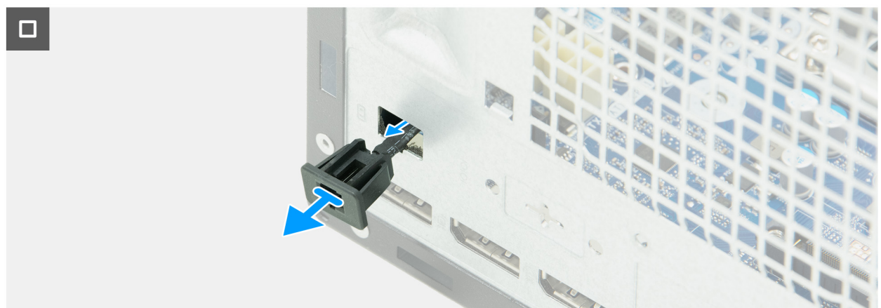
Figure 70. Removing the remote-power switch cable
